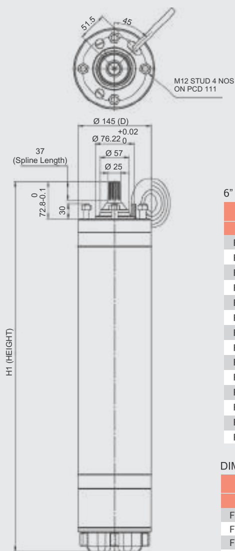
Dimensional Drawing
